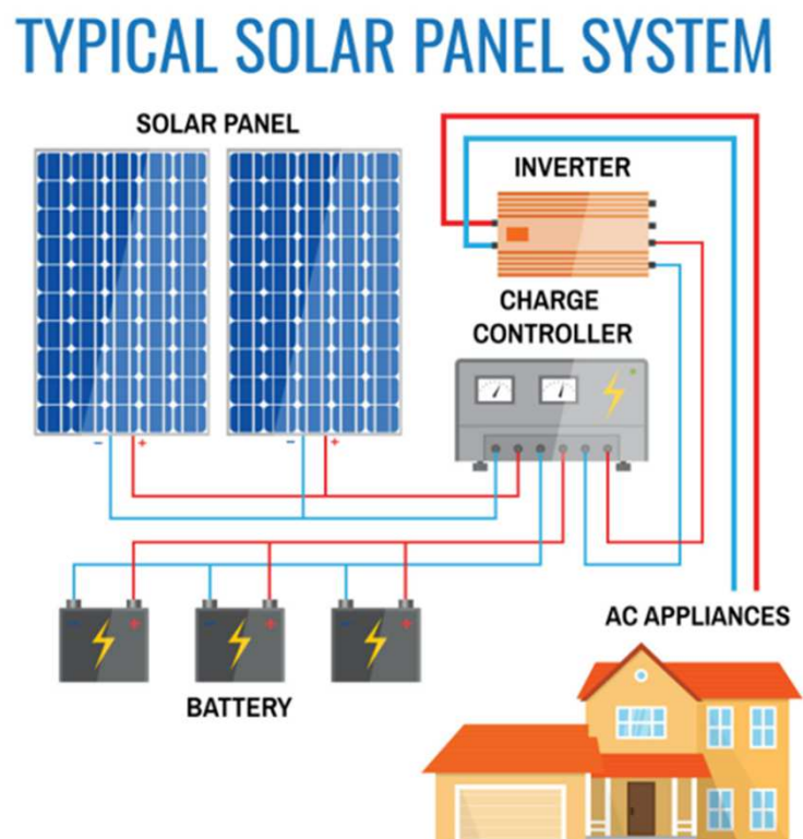
Solar Inverter System Illustration (Source: Herholdt's Group (Pty) Ltd.)
