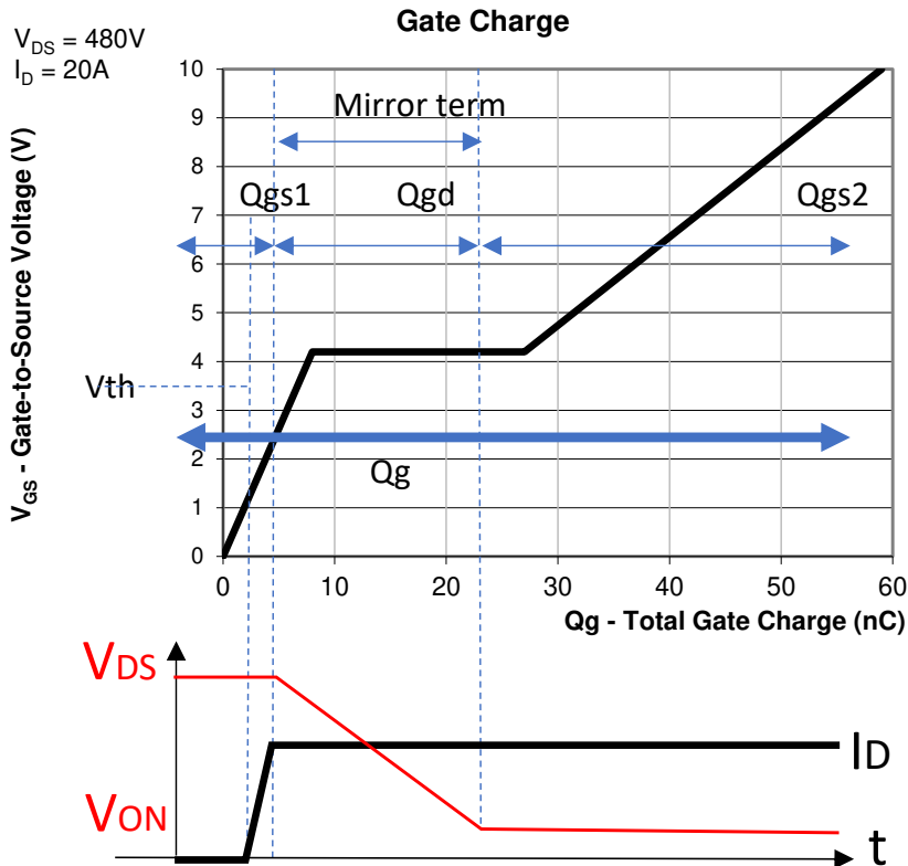
Fig.23 Gate Charge
